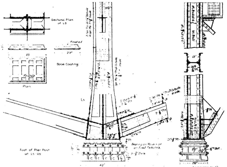
Details of Main Vertical Post, Portals and at Center of Channel Span.
