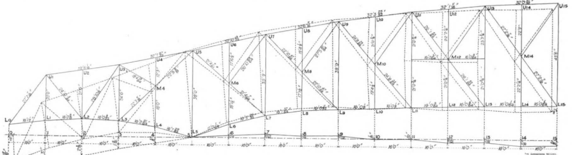
Dimensions and Deflections of Half the Bridge.
