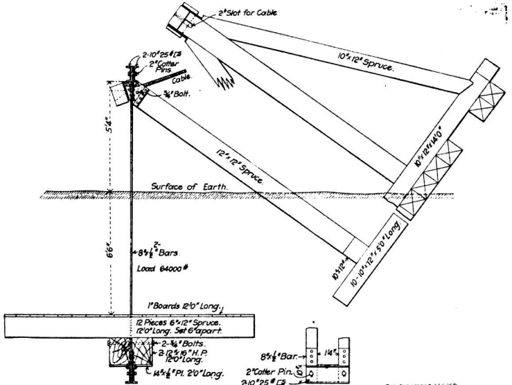
Anchorage for East End of Cableway.
