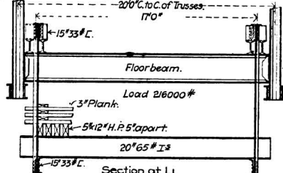
Suspended Platform for Temporary Counterweights for Erection Adjustment.
