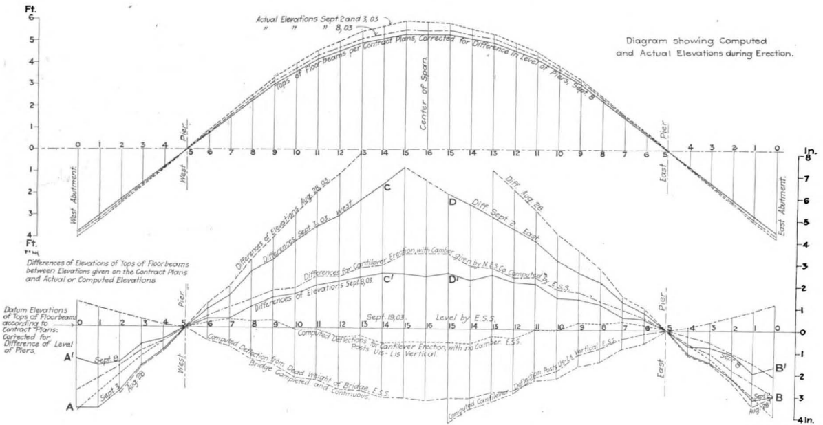
Diagram of Erection Elevations and Deflections.
