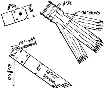
Knuckle Bearing at Top of West End Anchorage for Cableway.
