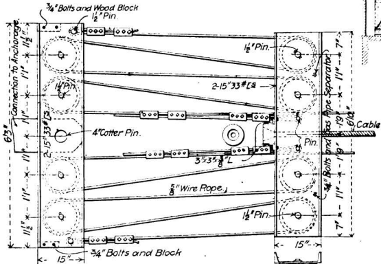
Adjustment Frame for Anchorage.
